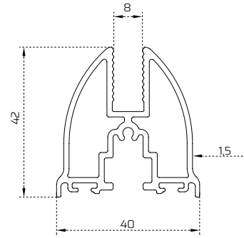
Foldtech 401 Baza Profili / Foldtech 401 Base Profile
