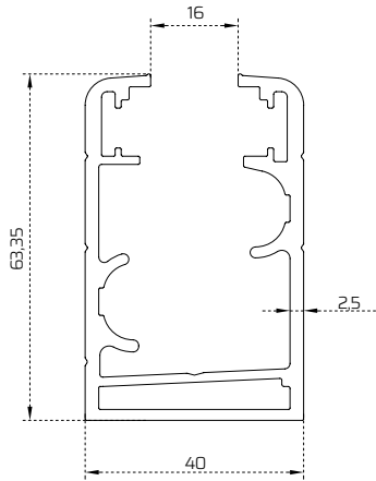
Kasa Profili / Case Profile
