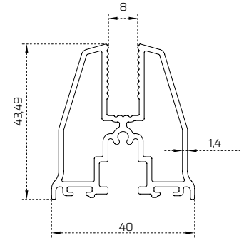
Foldtech 916 Baza Profili / Foldtech 916 Base Profile
