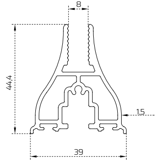
Foldtech 915 Baza Profili / Foldtech 915 Base Profile
