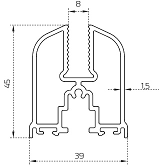
Foldtech 101 Baza Profili / Foldtech 101 Base Profile
